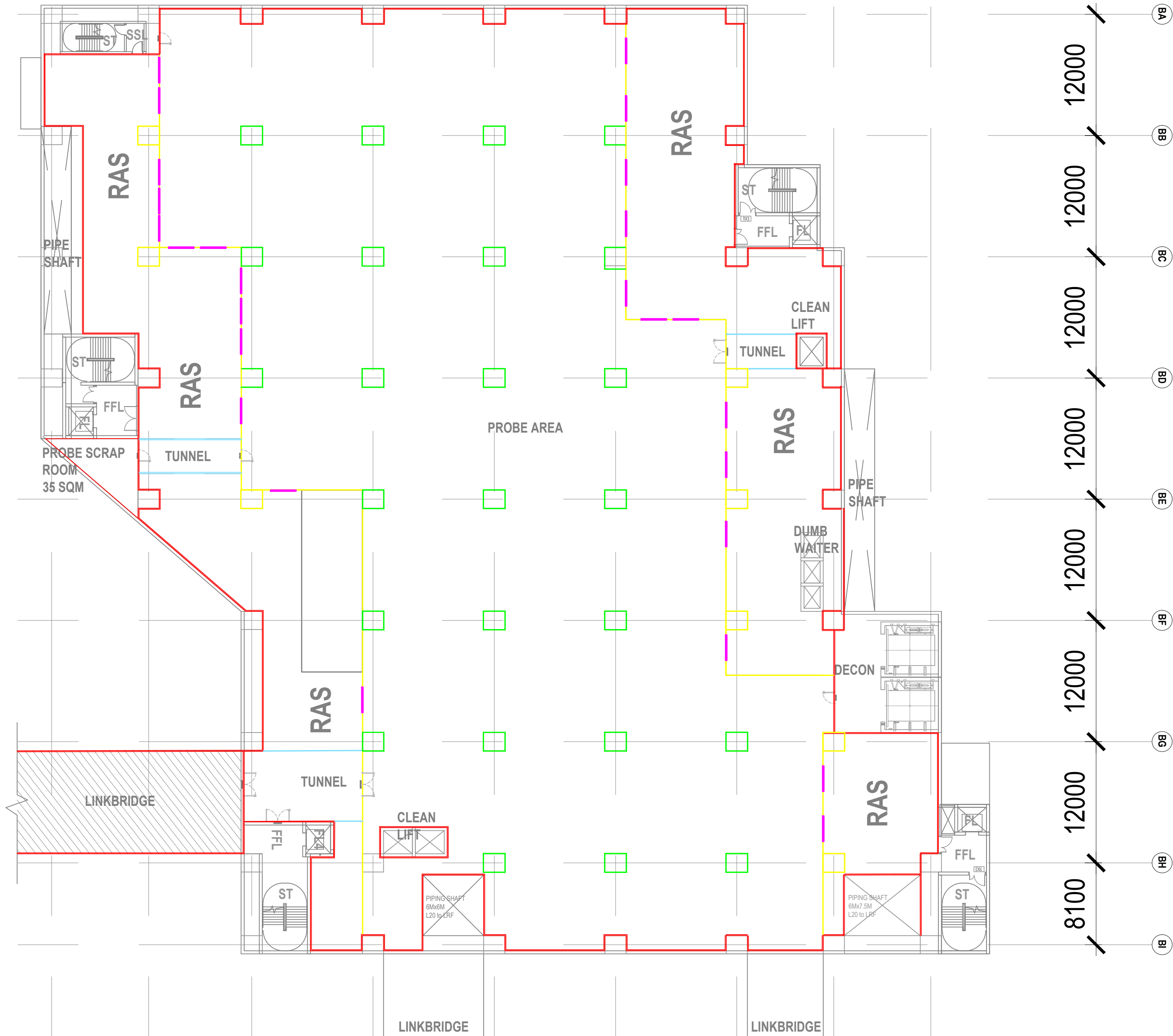
F10E2 L30 ,L40 ,L50, L70, L80, L100 PARTITION LAYOUT SCALE 1:300
